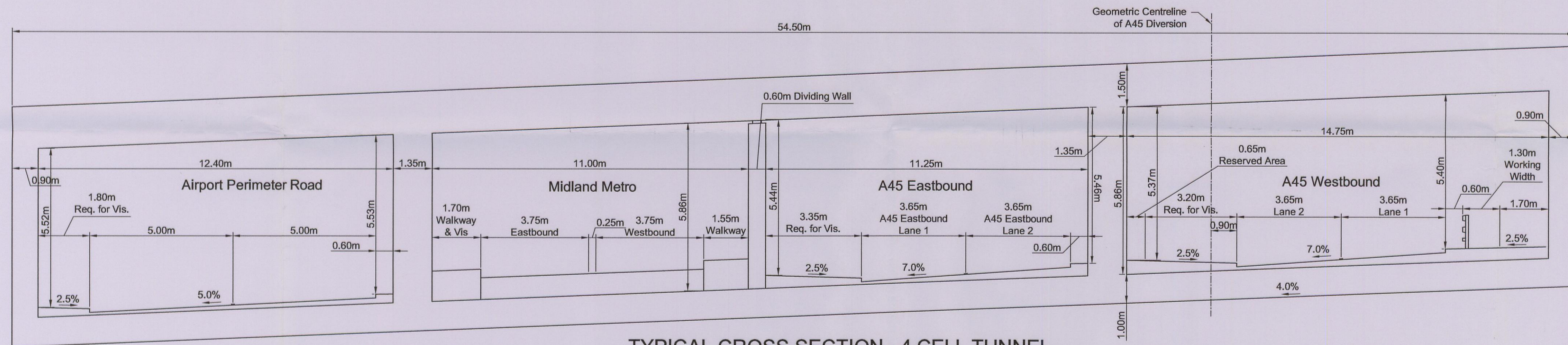
TYPICAL CROSS SECTION - 4 CELL TUNNEL (VIEWED FROM WEST) SCALE 1:100
